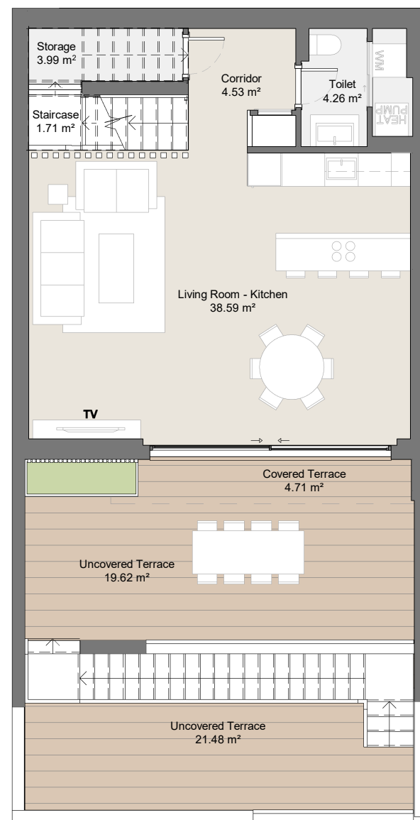
GROUND FLOOR
